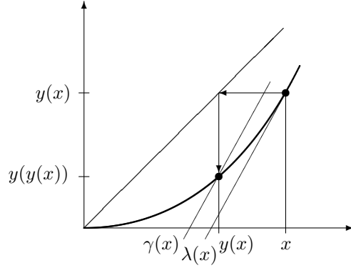
Figure 1: Original sub-tangent [\lambda(x), x] and scaled sub-tangent [\gamma(x), y(x)] .
