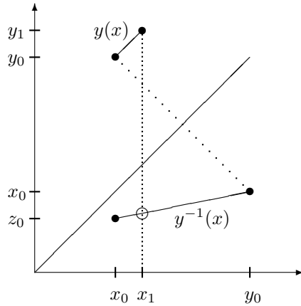
Figure 8: Initial linear segments of the solution function and its inverse with extra specification of the initial value z_0 of the inverse function. This allows to approximate the slope of the solution function at x_1 because y^{-1}(x_1) is now approximately given.
