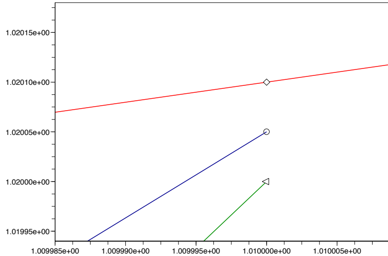
Figure 7: Exact solution function y(x) = x^2 (top curve) of y' = 2 \cdot (y^{-1})^2 in a small interval around x_1 = 1.01 with approximations starting at x_0 = y_0 = 1 for the conjoint forward iterations (middle curve) and individual forward computations based on the function and its inverse (bottom curve).
