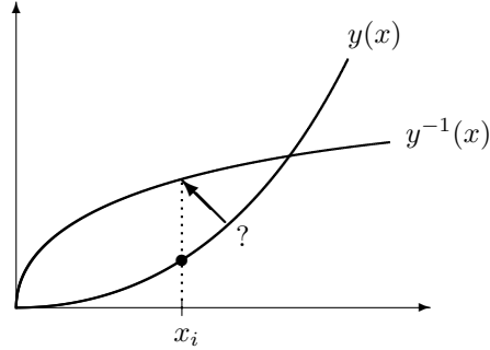
Figure 4: Reasonably approximating the value of the inverse solution function at x_i , which would then computations allow to use the value F(y^{-1}(x_i), x_i) , requires to (approximately) know the function values at larger arguments.
