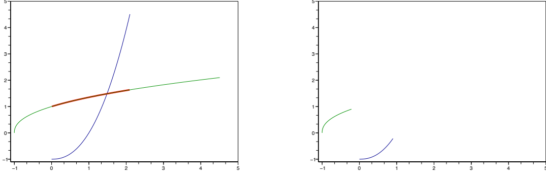
Figure 2: Function y(x) = x^{2.3} - 1 over domain [x_0, x_n] = [0, 2.1] (left) and [x_0, x_n] = [0, 0.9] (right) with inverses. For the larger function domain, the inverse is also computed over the approximation domain by Test-and-invert (bold function segment). In the other case, the approximation domain is empty (right) since the largest value of the function is smaller than the smallest value of the inverse.
