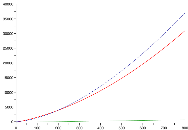
Figure 5: Solution function (bold curve) over Dom = [0, 800] computed by the fixed point method for y'(x) = y^{-1}(x) with initial boundary value y(0) = -200 . Initialization was obtained by the linear function y(x) = x - 200 (thin curve). Included for comparison is the golden section function y(x) = (1/g)^{1/g} \cdot x^g solving the problem for the initial boundary value y(0) = 0 (dashed curve).
