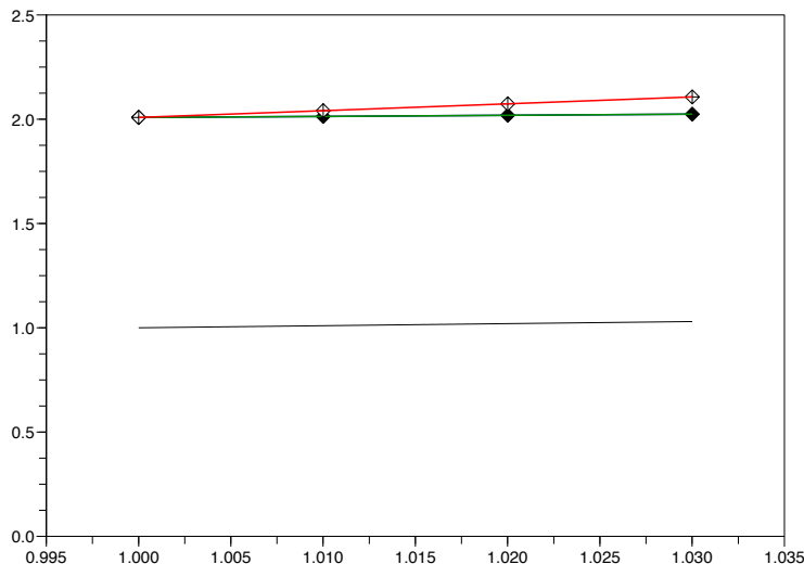
Figure 9: Solution function y(x) = (5/g)^{1/g} \cdot x^g (top curve) and forward approximation (middle curve) with exact boundary value y_0 = y(1) and value z_0 = 0.1 for the ODEI y' = 5 \cdot y^{-1} over the interval [x_0, x_3] = [1, 1.03] . Relative approximation errors at the support points x_1, x_2 and x_3 are 1.35%, 2.69% and 3.89% respectively. The error values are identical – up to three decimals – for the pure forward method and for the forward method with overwriting. Solutions lie above the diagonal (bottom curve).
