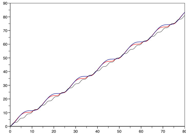
Figure 10: Solution (bold curve, partially occluded) over Dom = [0, 80] for y'(x) = \sin(y^{-1}(x)) + 1 with initial boundary value y(0) = 0 as in figure 6 (left). Linearly induced approximating functions y_{lin}(x) = x - 2 \cdot \cos(0.5x) + 2 for \alpha = 0.5 (bold curve, same frequency and "mostly" above the solution) and y_{lin}(x) = x - 0.5 \cdot \cos(2x) - 0.5 for \alpha = 2 (thin, high frequency curve).
