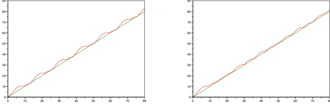
Figure 6: Solutions (bold curves) over Dom = [0, 80] computed by the fixed point method for y'(x) = \sin(y^{-1}(x)) + 1 (left) and y'(x) = \sin(y^{-1}(x)) \cdot \cos(0.1 \cdot y^{-1}(x)) + 1 both with initial boundary value y(0) = 0 and initialization function y(x) = x (thin curves).
