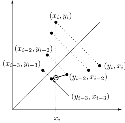
Figure 3: Points on the function and on the inverse function with correspondences (slanted dotted lines). The value of the inverse function at support point x_i is, in this case, linearly interpolated from the values y_{i-3} and y_{i-2} so that j = i - 3 .
